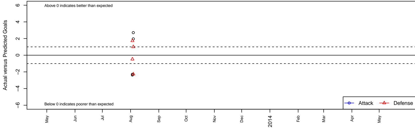
Lynden Ladies G01 Dots are actual minus expected GF (blue circles) and GA (red triangles). Blue line is smoothed change in attack strength. Red is smoothed change in defense strength.
